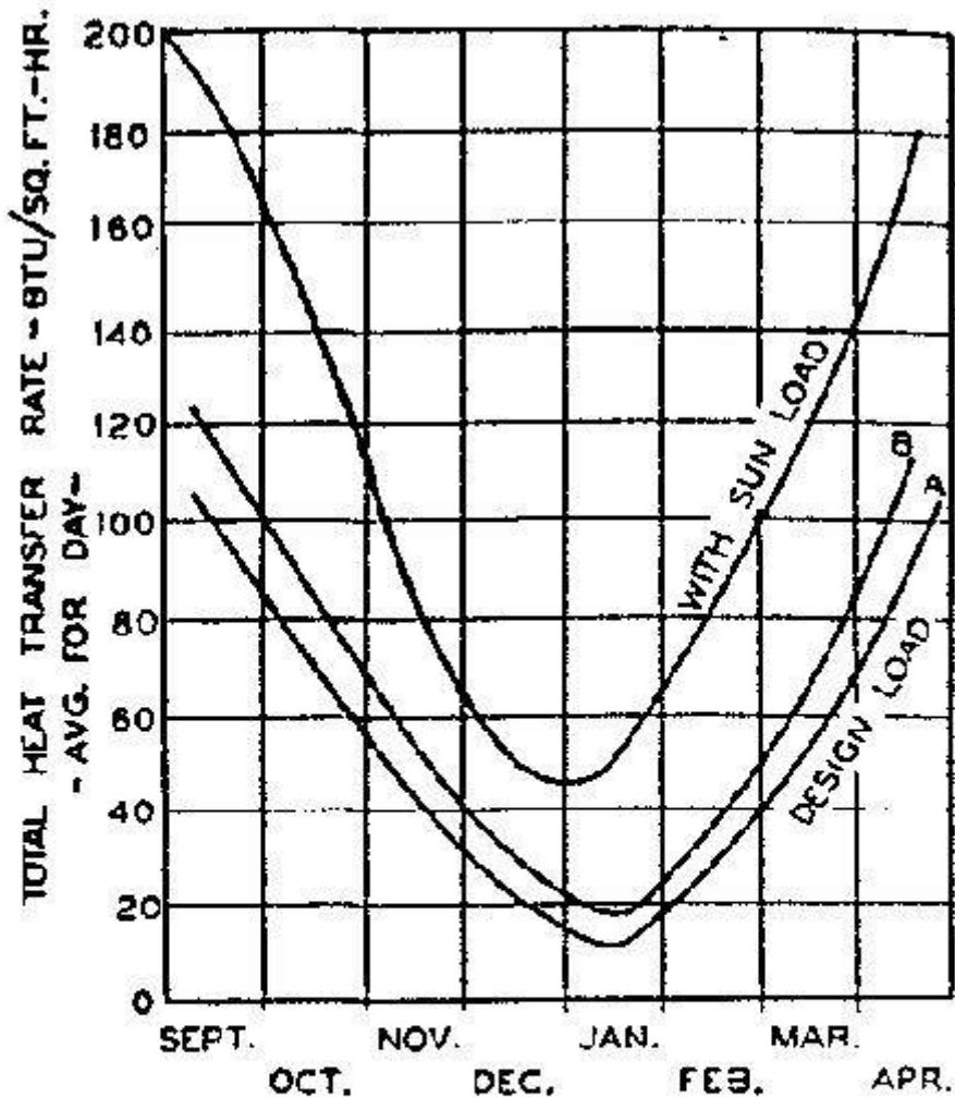
Fig. 15 t . Maximum Noontime Load on Outdoor Skating Surface on a Clear Day—Sum of Ground, Air and Sun Loads. Lower Curve is Recommended Design Value Counting Upon Storage Effect of Ice and Equipment When Machine is Run Steadily. A is for Cloudy Day and B for Sunny Day.
